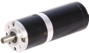
60JX300K/60ZY105直流行星减速电机 减速器直径60mm，输出转矩30N.m Model: 60JX300K/60ZY105 (DC Planetary Gear Motor) Gearbox OD: 60mm; Output Torque: 30N.m
